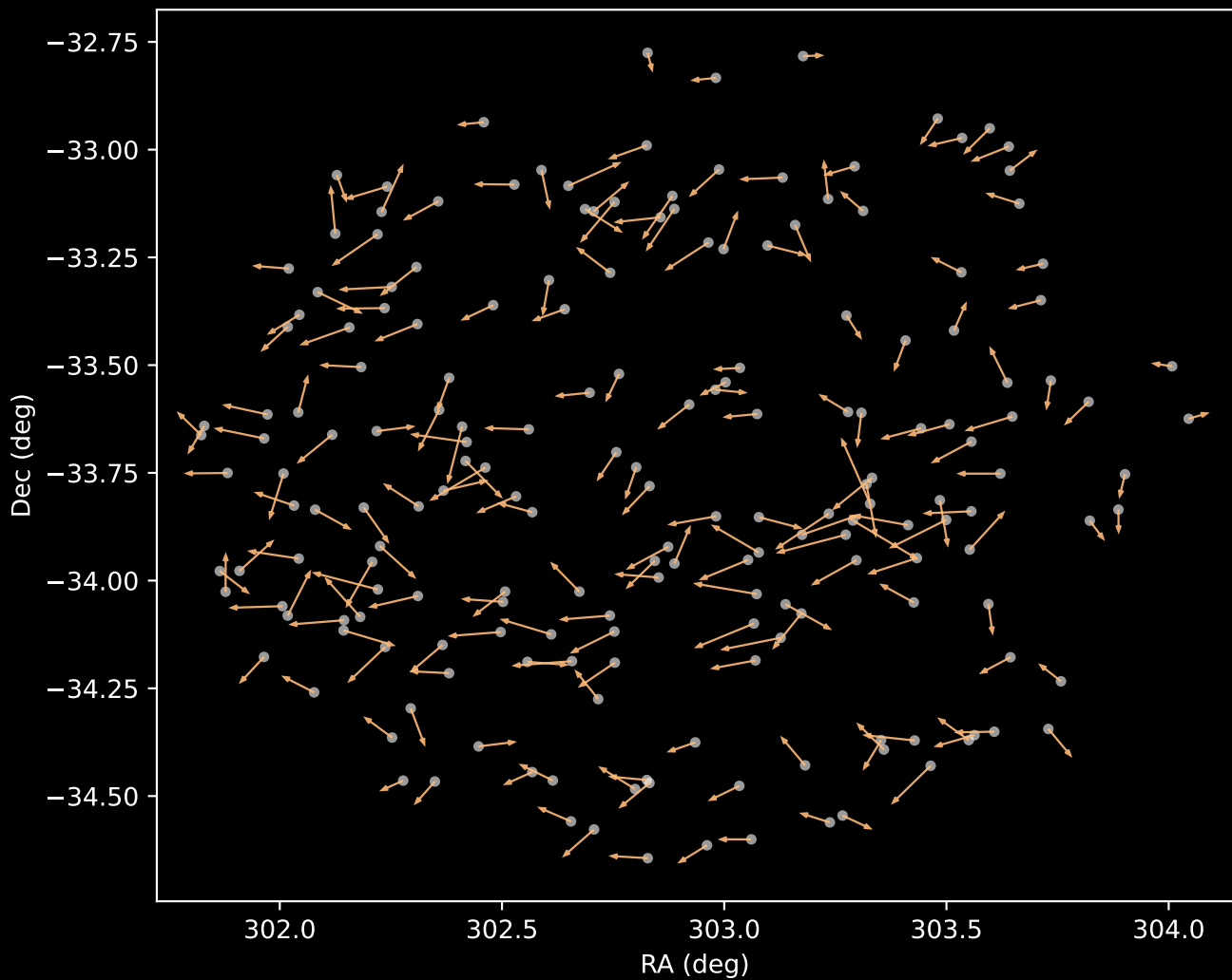
APOGEE DR17 Cluster 3 Proper Motion Vectors (n=192)
