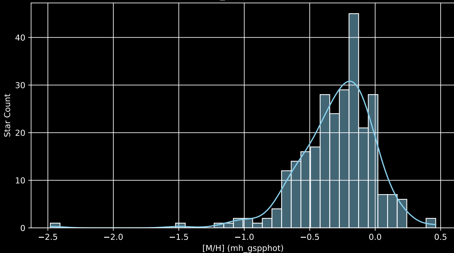
APOGEE DR17 Field: [313+29 [M/H] (mh_gspphot) (n= 271)
