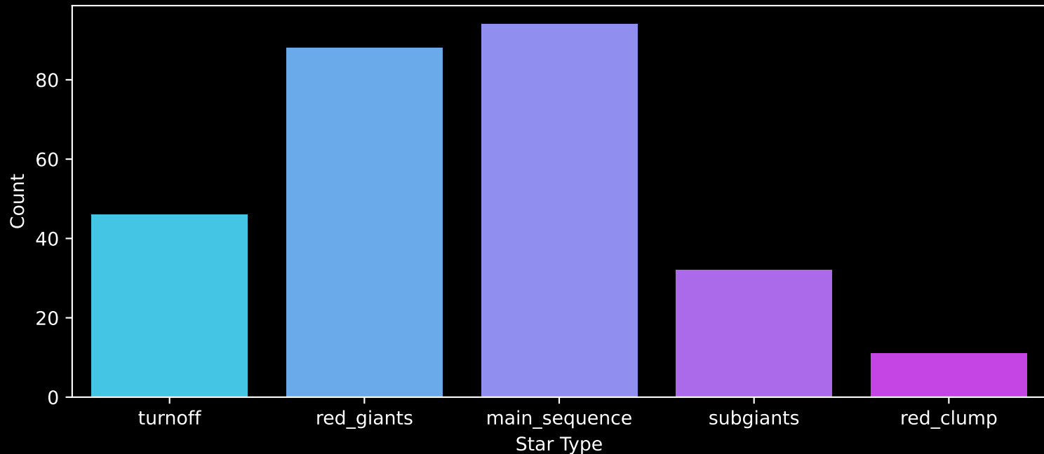
APOGEE DR17 Field: [313+29] Count plot of Star Type
