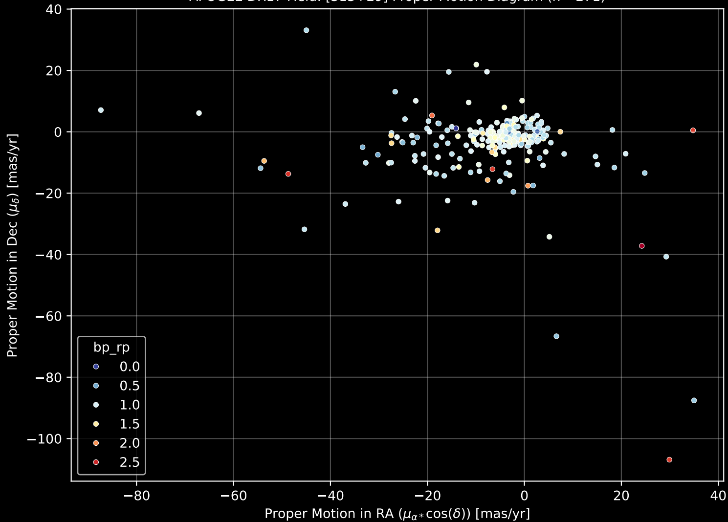
APOGEE DR17 Field: [313+29] Proper Motion Diagram (n= 271)
