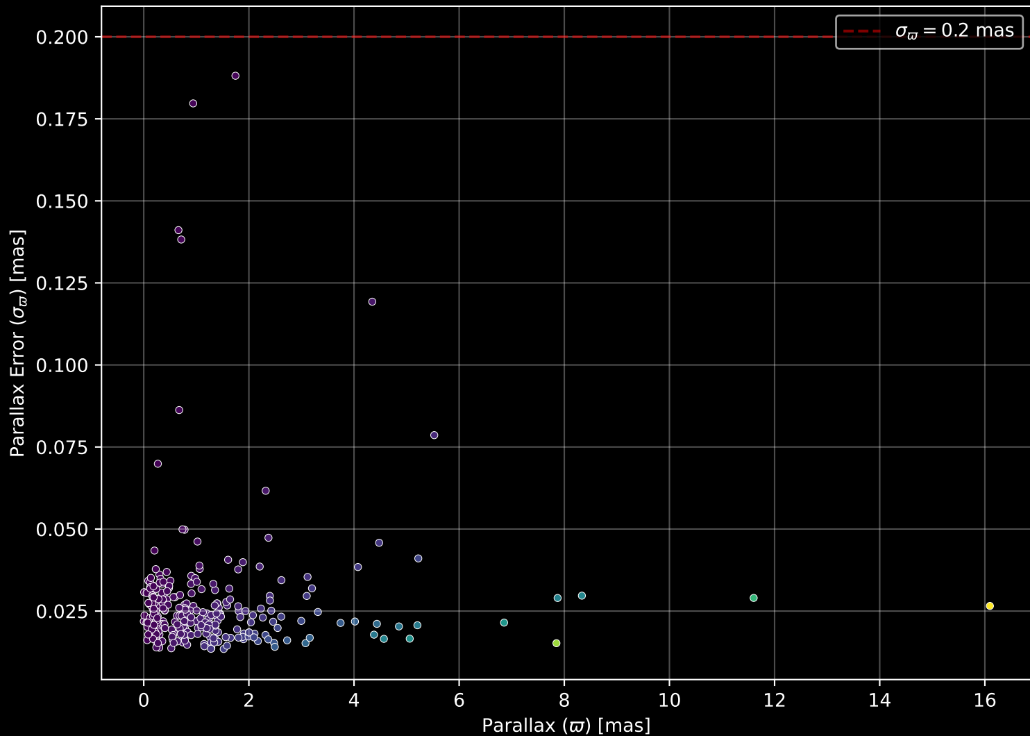
APOGEE DR17 Field: [313+29] Parallax Quality (n= 271)
