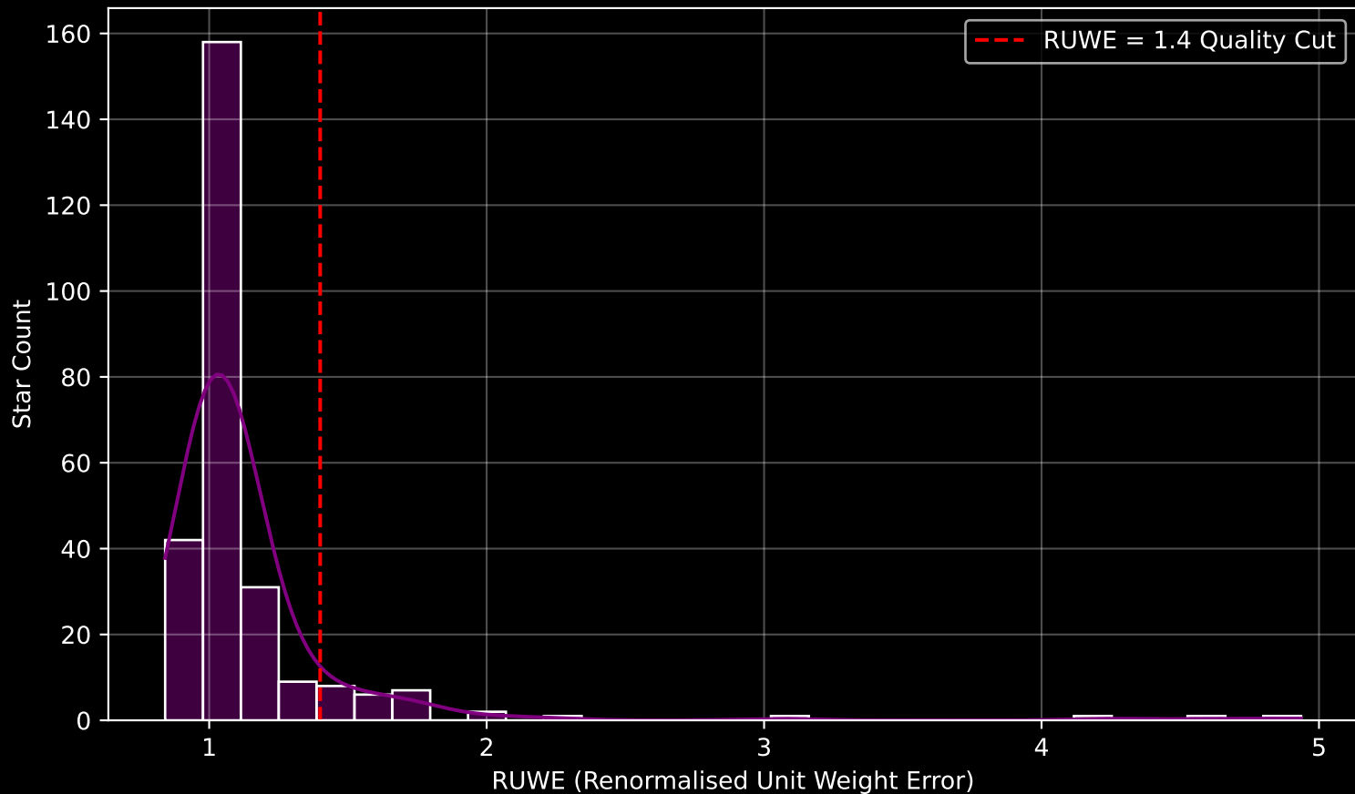
GAPOGEE DR17 Field [313+29] RUWE Distribution (n= 268)
